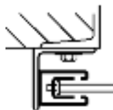
Face of Wall to Steel
