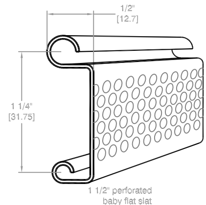
CURTAIN DETAIL
