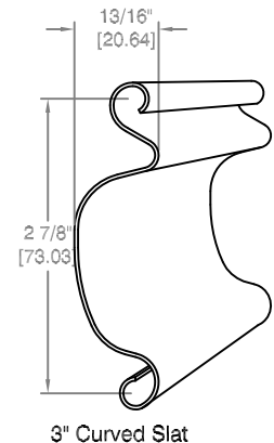
CURTAIN DETAILS
