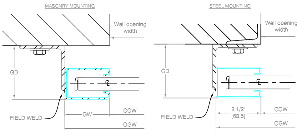
GUIDE SECTION B - B
