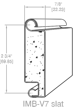
SLAT DETAIL
