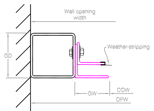
TUBE MOUNTED
