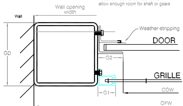
VERTICAL SECTION A - A
