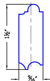
SLAT PROFILE
