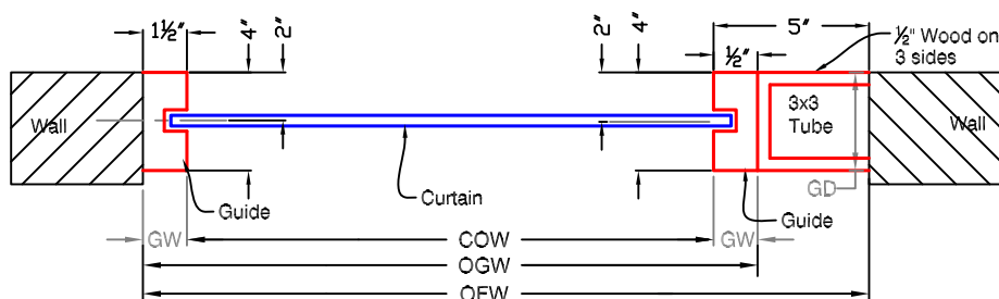
GUIDE SECTION
