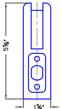
BBAR PROFILE
