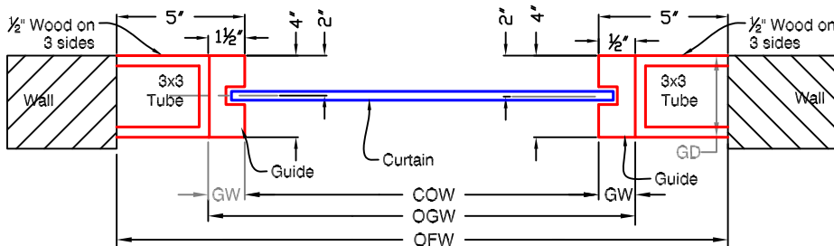
GUIDE SECTION
