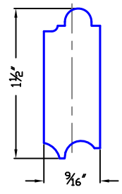
SLAT PROFILE
