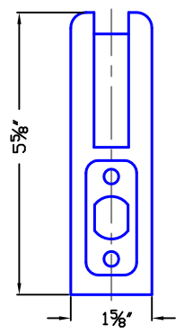
BBAR PROFILE
