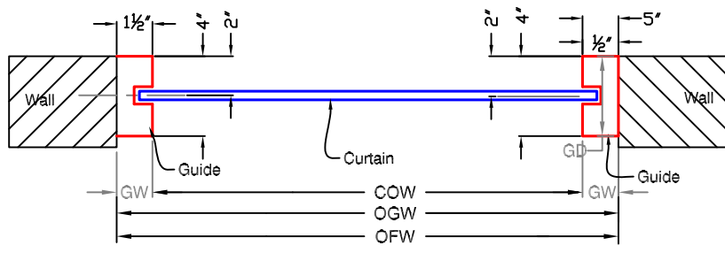
GUIDE SECTION
