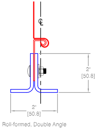
Roll-formed, Double Angle
