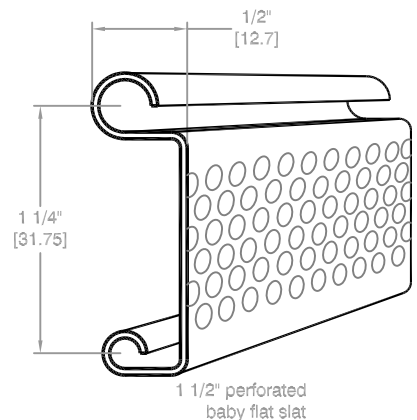
CURTAIN DETAIL
