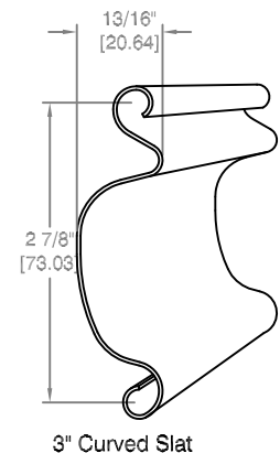
CURTAIN DETAILS
