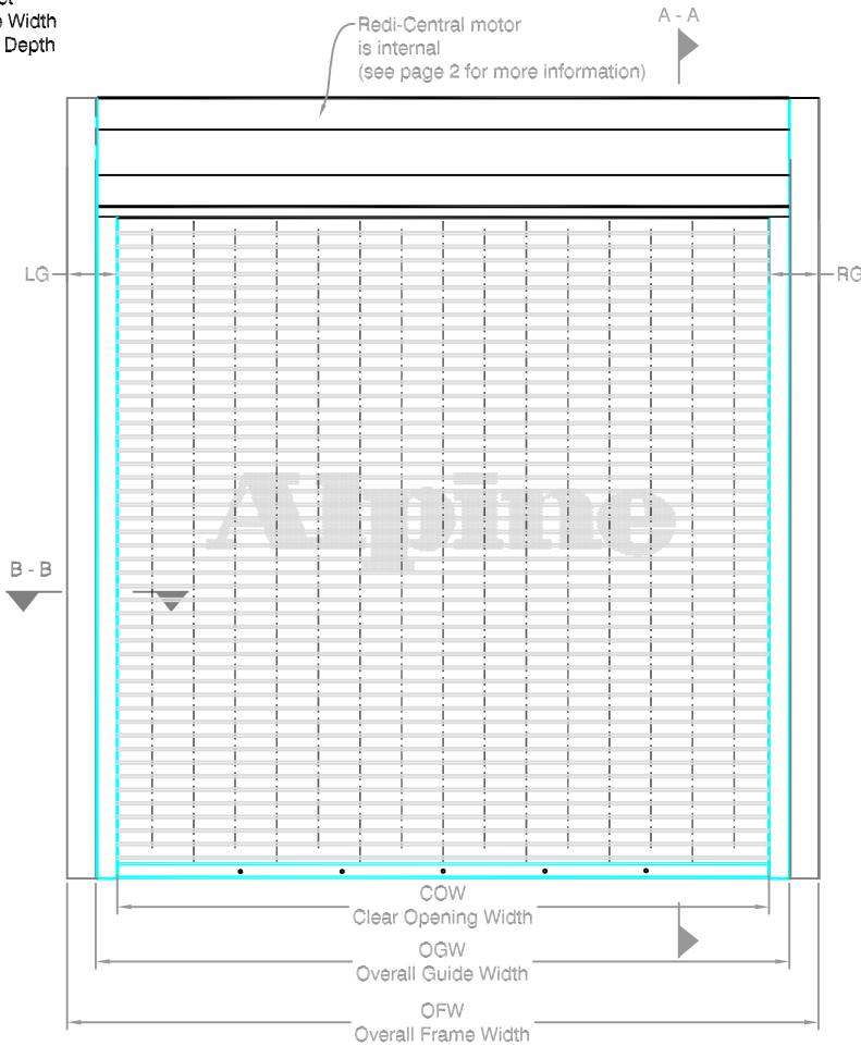
COIL SIDE ELEVATION
