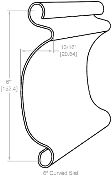
6" Curved Slat
