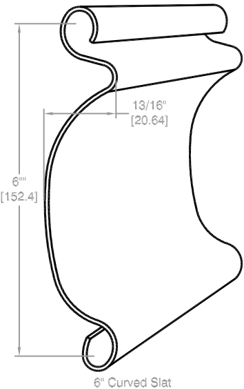
CURTAIN DETAIL
