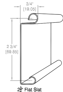
CURTAIN DETAIL
