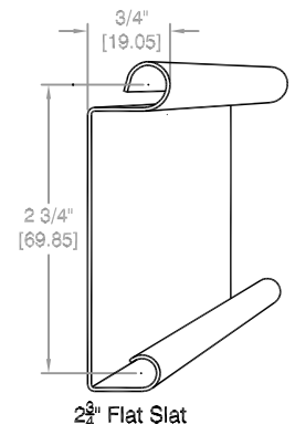
SLAT DETAIL
