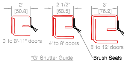
GUIDE DETAIL
