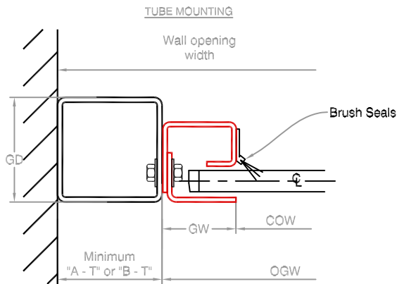
GUIDE SECTION B - B
