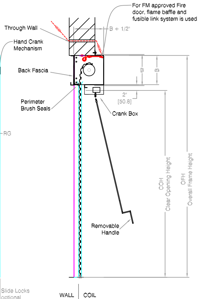
VERTICAL SECTION A - A
