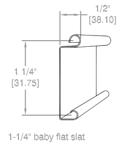
CURTAIN DETAIL
