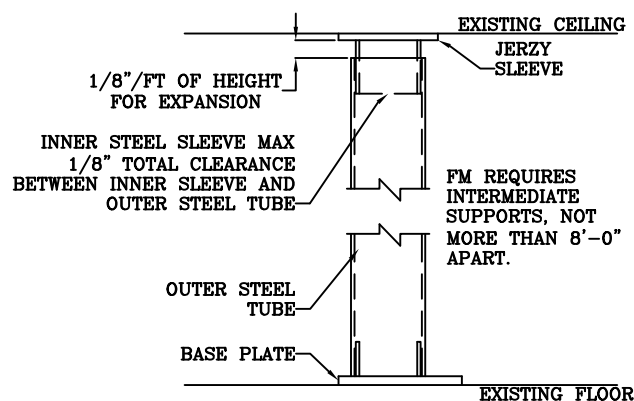
TUBE MOUNTING FOR FIRE DOORS TO ALLOW FOR HEAT EXPANSION
