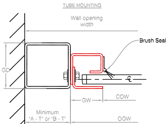
GUIDE SECTION B - B
