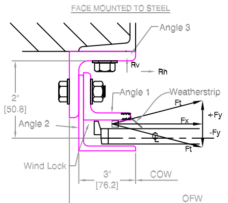
GUIDE DETAILS
