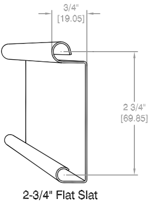
CURTAIN DETAIL
