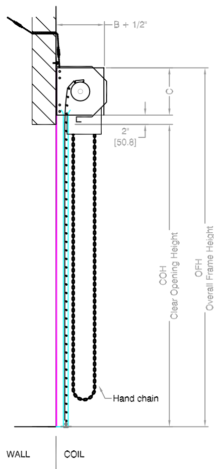
VERTICAL SECTION A - A
