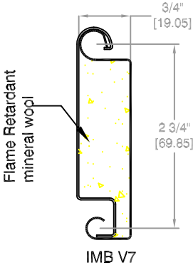
CURTAIN DETAIL
