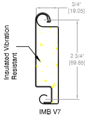
CURTAIN DETAIL
