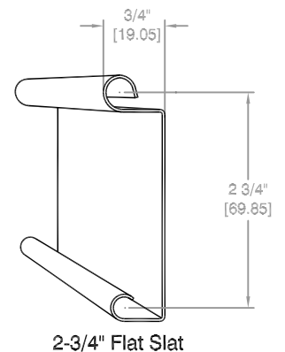
CURTAIN DETAIL
