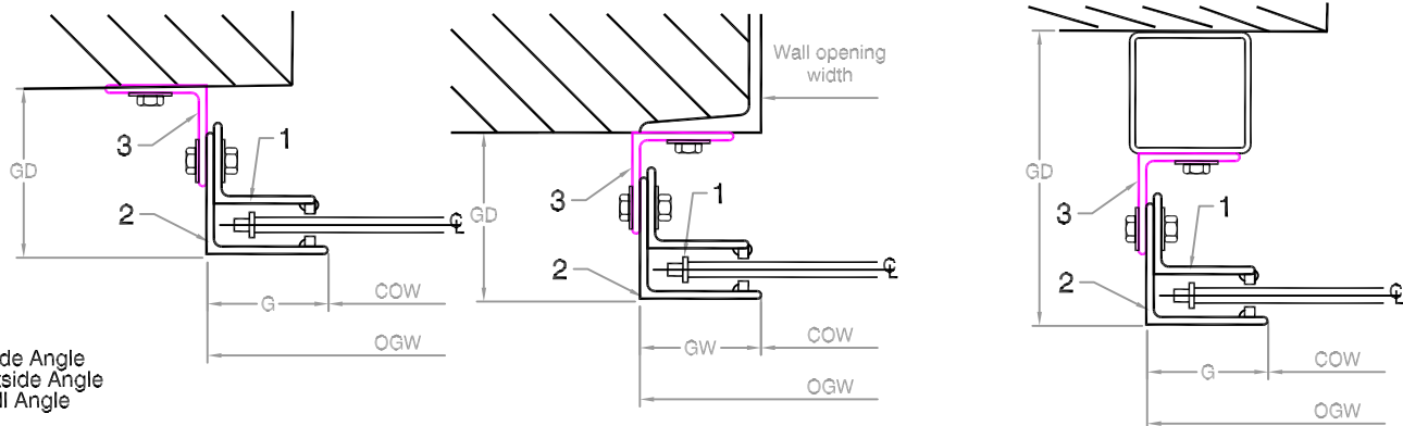
GUIDE SECTION B - B
