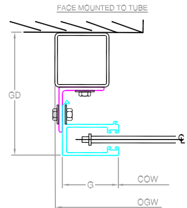
VERTICAL SECTION A - A
