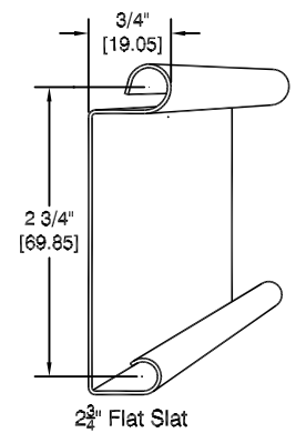
CURTAIN DETAIL
