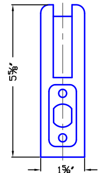
BBAR PROFILE
