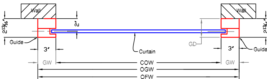
GUIDE SECTION
