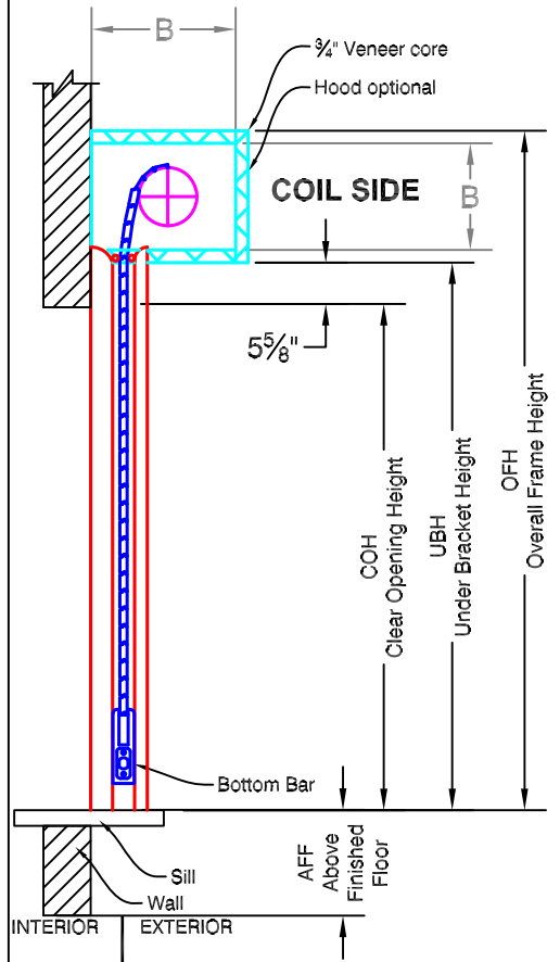
VERTICAL SECTION A - A
