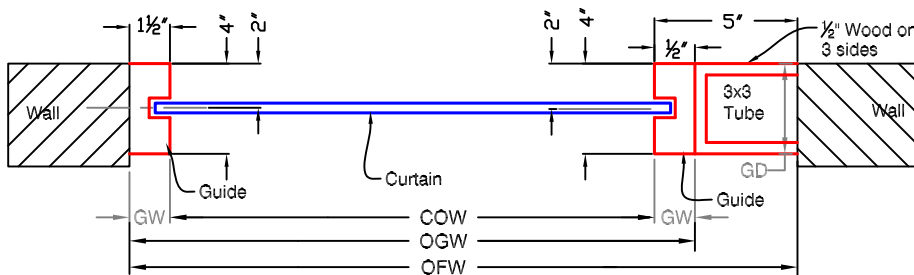
GUIDE SECTION
