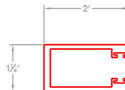
Aluminum Guide (between jambs)
