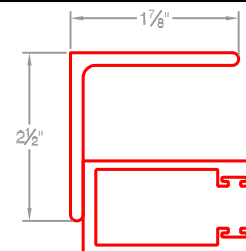
Aluminum Guide (face of wall)
