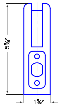
BBAR PROFILE
