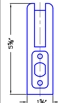
BBAR PROFILE
