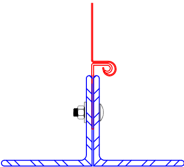
Structural Steel Double Angle
