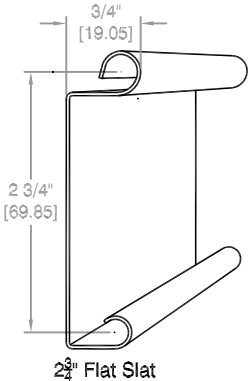
2 3/4" Flat Slat
