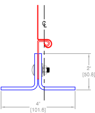
Roll-formed, Double Angle
