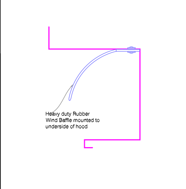
CURTAIN DETAIL OBSTACLE EDGES AVAILABLE WIND BAFFLE DETAIL
