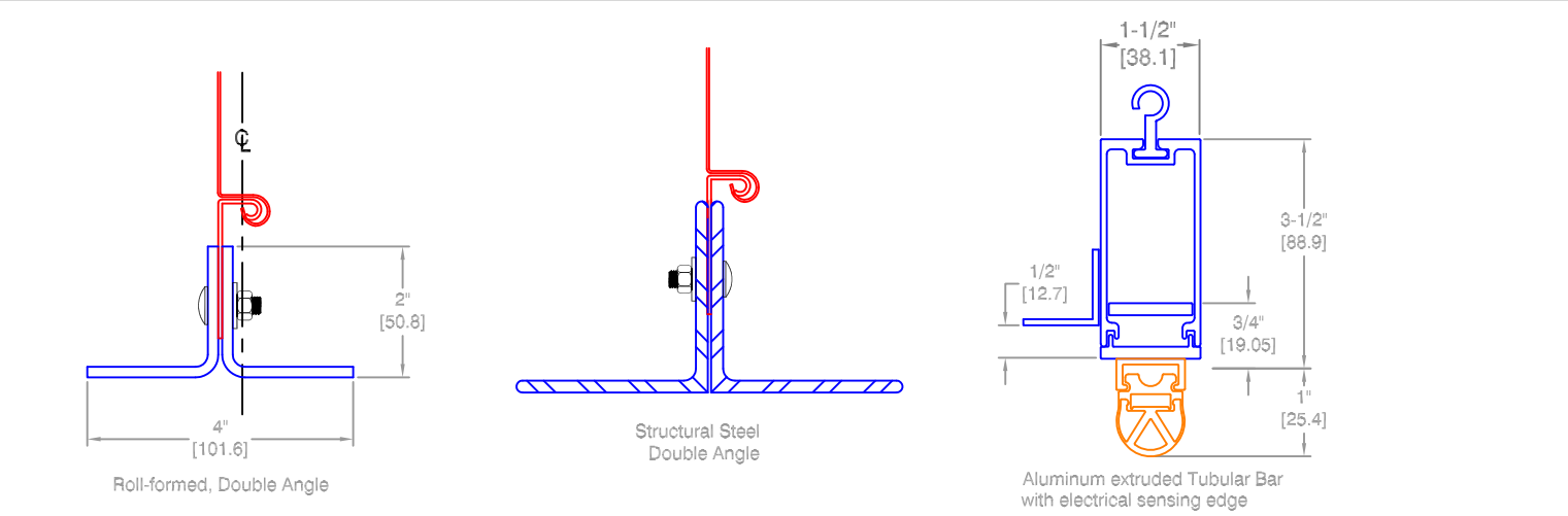
BOTTOM BAR DETAIL
