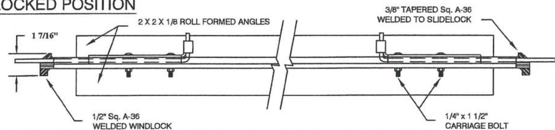
SLIDE LOCK
