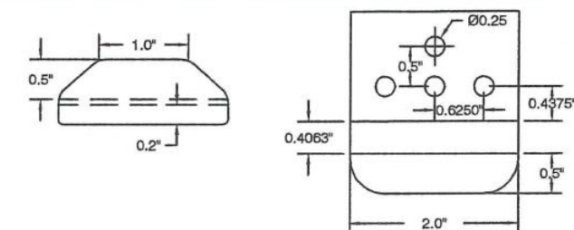
WINDLOCK
