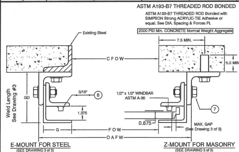
GUIDE SECTION
