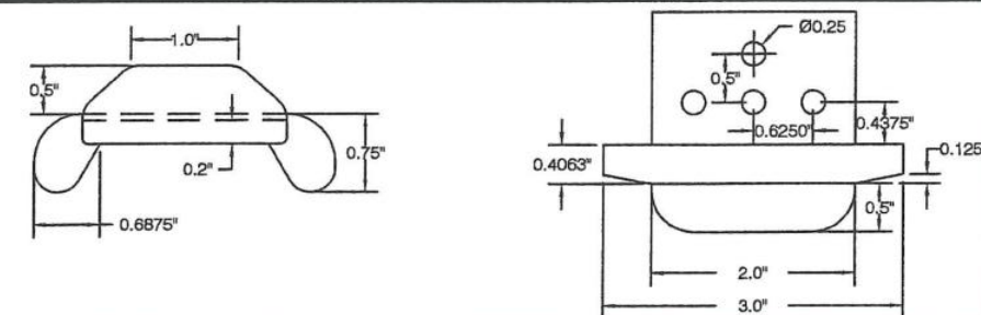
WINDLOCK / ENDLOCK
