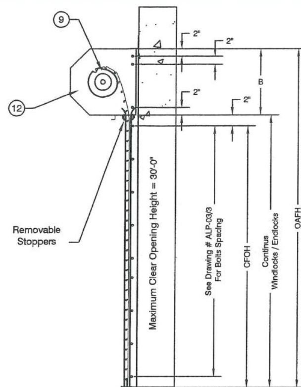
VERTICAL SECTION
