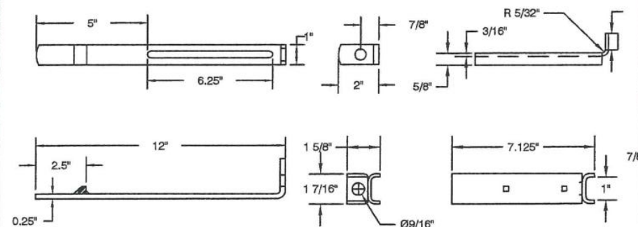
WINDLOCK / ENDLOCK
