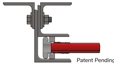
Heavy Duty Structural Guides Made from high strength steel Shown with Dual Riot-Lock™
